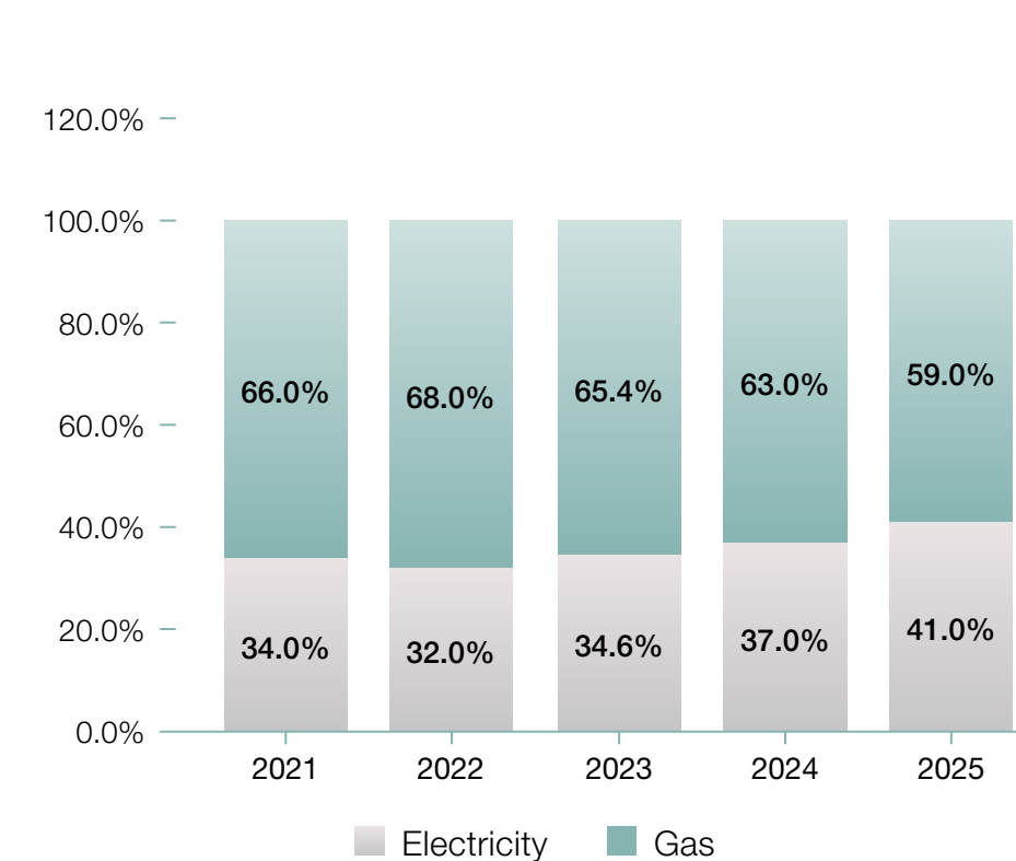
Energy by Source for Motorcycle Production
