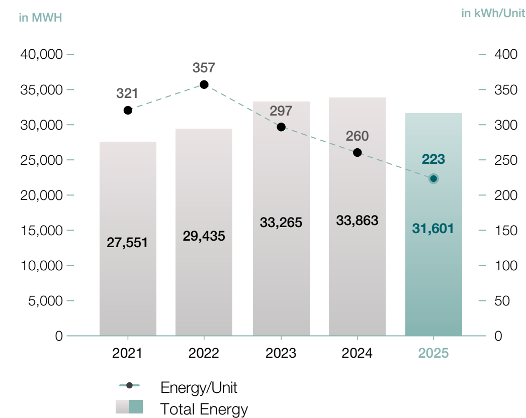
Energy Consumption for Motorcycle Production
