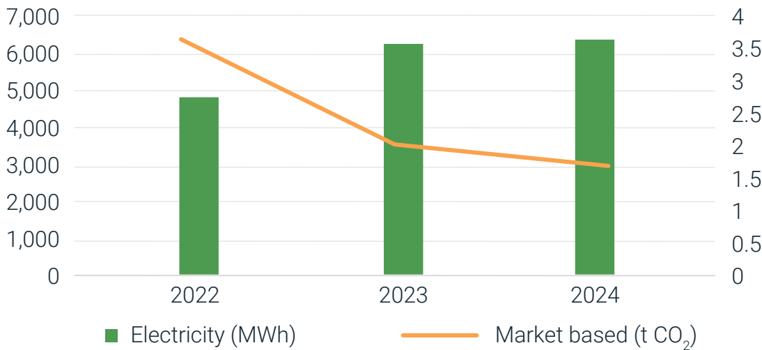
Electricity consumption vs market-based emissions
