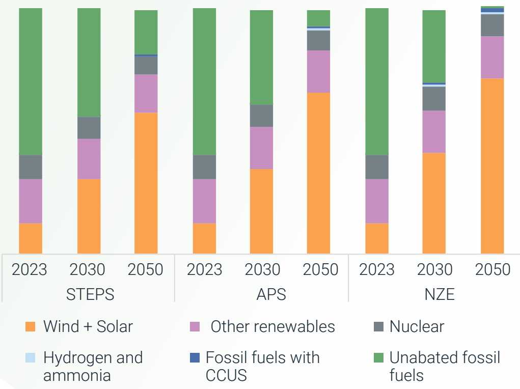
Distribution of electricity generation, WEO 2024
